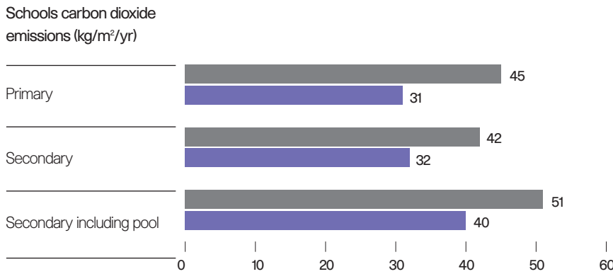
Figure 15 Energy use benchmarks for schools (Source: CIBSE Guide F)
